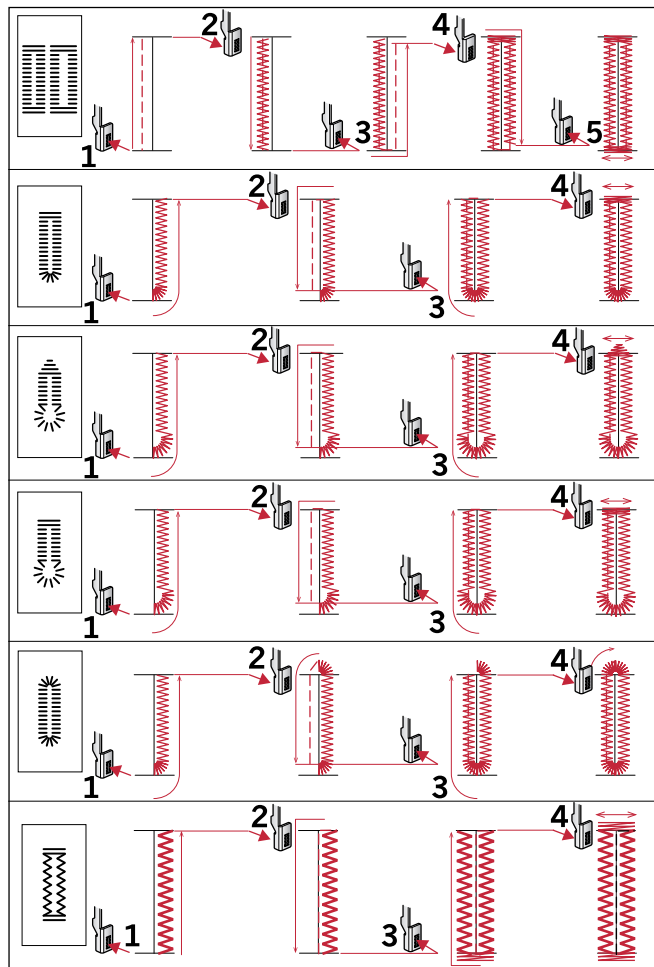
Sewing sequences for buttonhole stitches 25–31.
